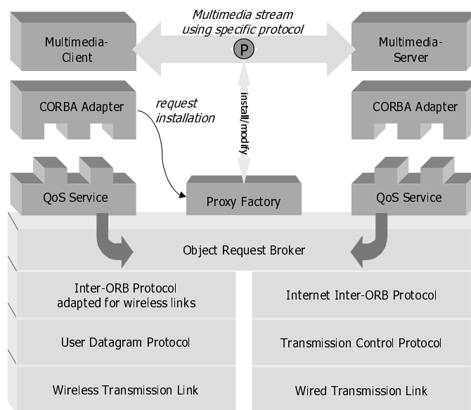
Figure 2: An Overview of the RAPP Architecture
