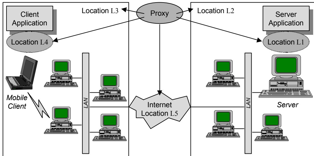
Figure 3. Options of Proxy Placement
